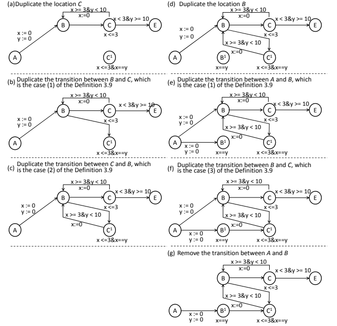
Fig. 15 The Refinement Process for the Path in Fig. 7
