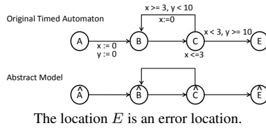
Fig. 4 Example of a Timed Automaton and its Abstract Model
