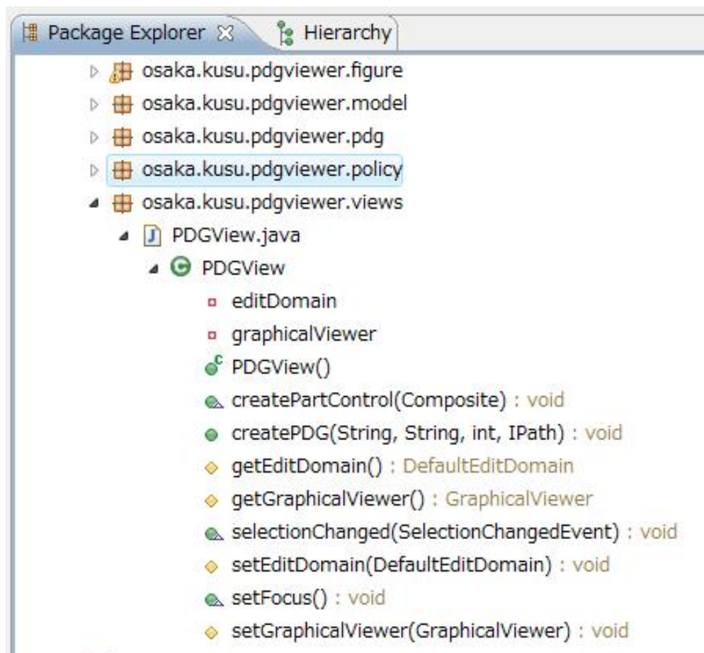
Figure 7: Package Explorer
