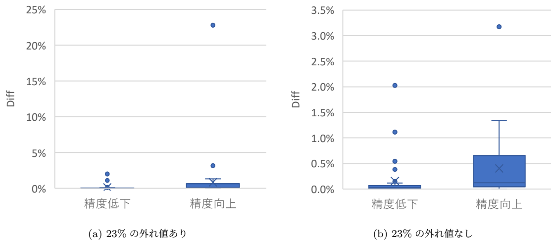
図 11 SBFL と GASBFL の Diff
