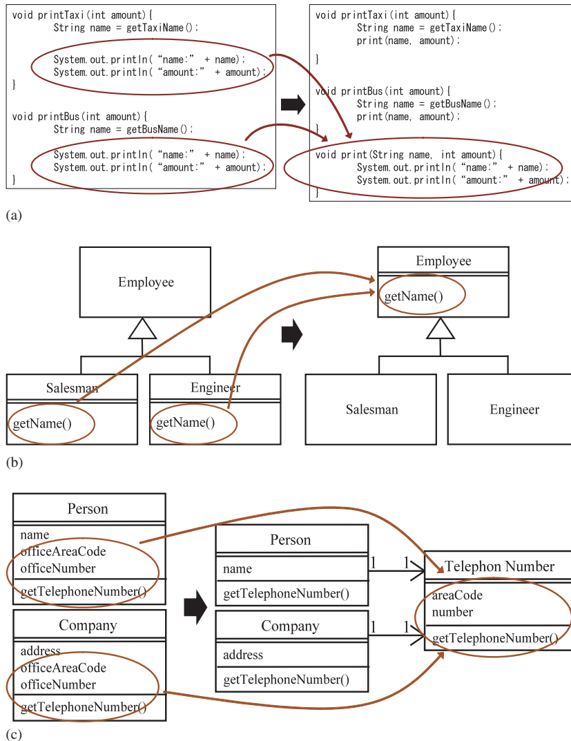
Figure 3. Examples for merging code clones: (a) Example of CASE1; (b) Example of CASE2; and (c) Example of CASE3.
