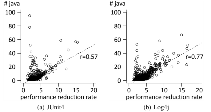
Fig. 4: Relationship between performance reduction rate and number of java files
