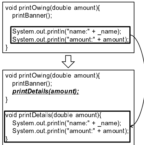
図5 Extract Method
