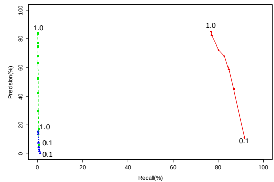
(b) jEdit
