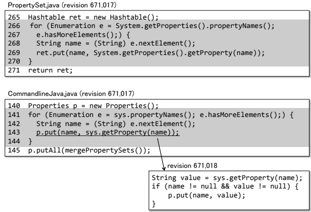
Figure 11: Code where an unintended inconsistency occurred
