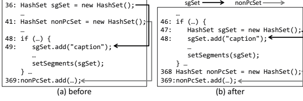
Figure 1. Motivating Example
