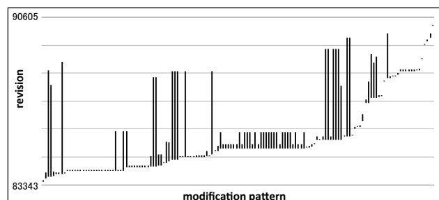
(a) HTTPD
