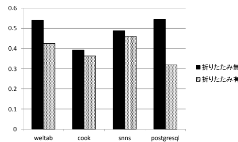
(c) goodrecall
